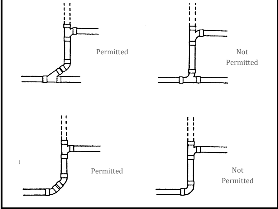
FIGURE 7: Permitted Use of Sanitary "T" (TY) Fittings
