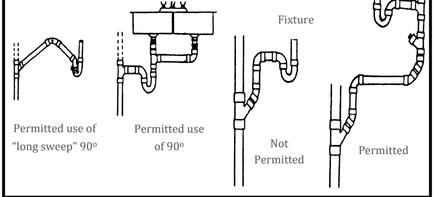
FIGURE 8: Permitted Use of Sanitary "T" (TY) Fittings - Exceptions
