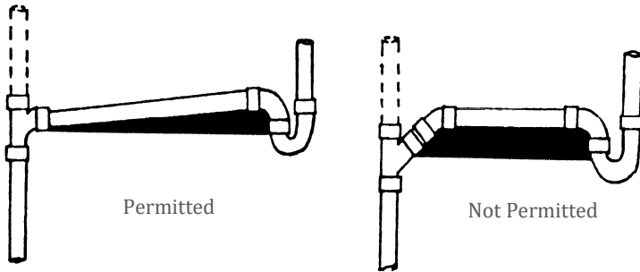
FIGURE 3: Fall of Fixture Trap
